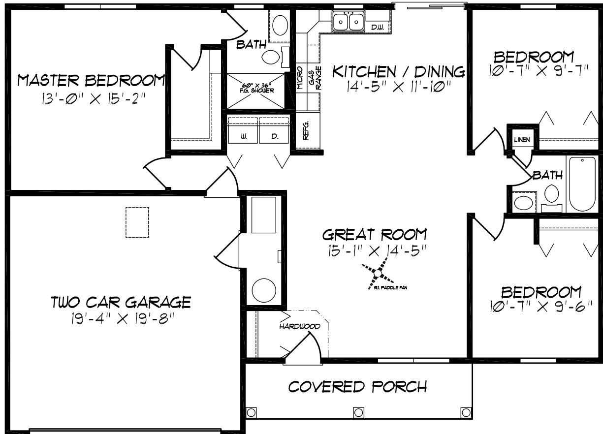
FLOOR PLAN
