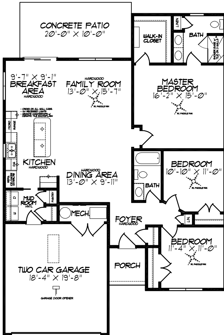
FLOOR PLAN 9' CEILING HEIGHT
