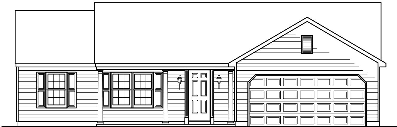
FRONT ELEVATION
