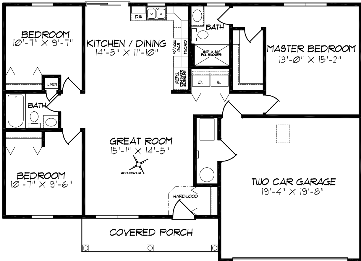
FLOOR PLAN
