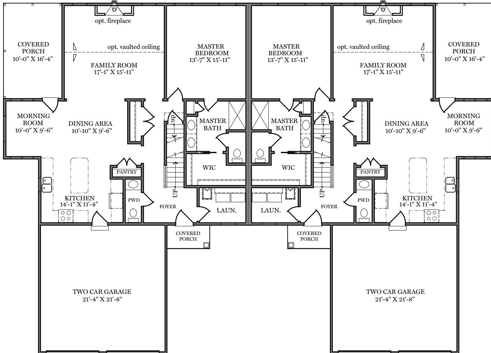
First Floor Plan - 1,364 sf "TARRAGON" (full basement option shown)
