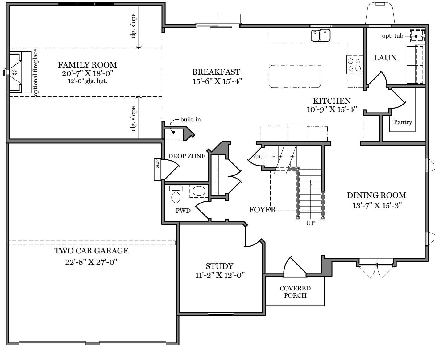
First Floor Plan - 1,651 sf "MAGNOLIA"
