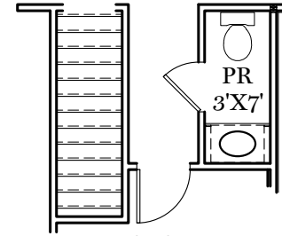
OPTIONAL POWDER ROOM
