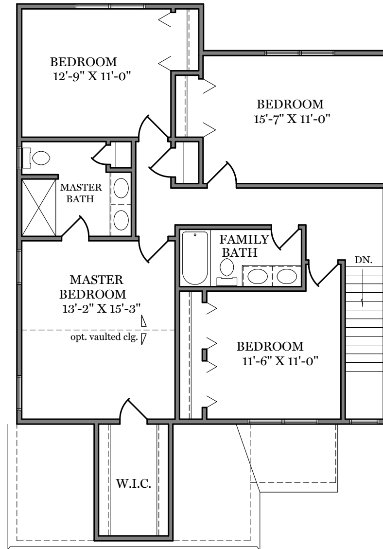
Second Floor Plan - 1,155 sf "JAMESON"
