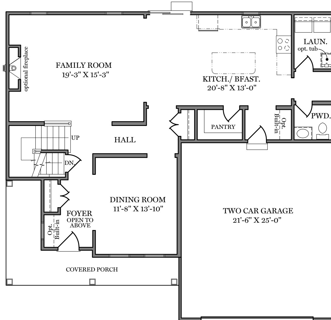
First Floor Plan - 1,223 sf "GLENWOOD"
