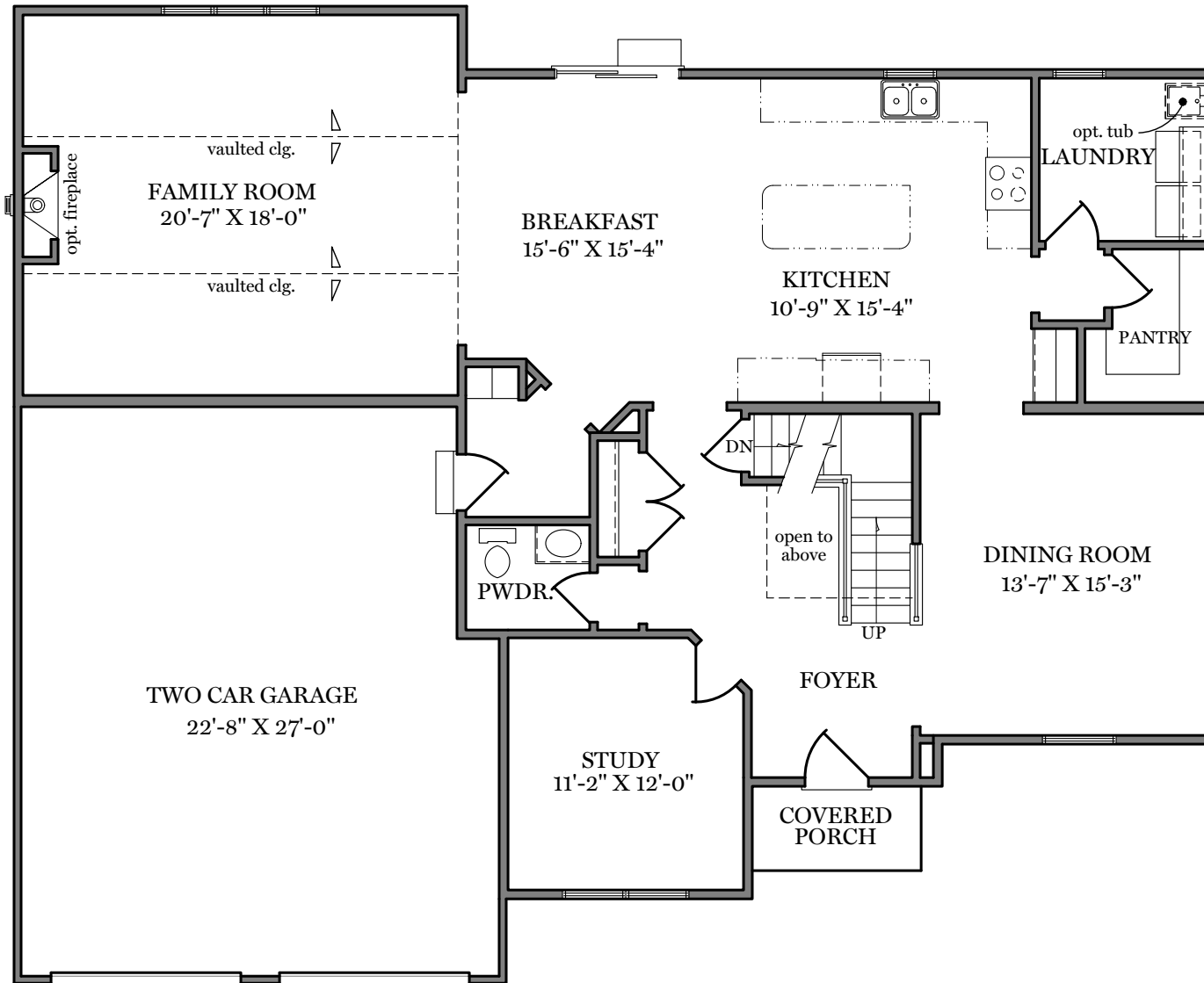
First Floor Plan - 1,651 sf "MAGNOLIA"
