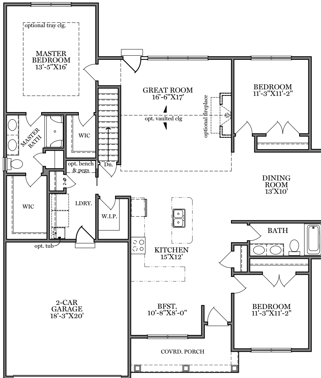
First Floor Plan - 1,829 sf "HENSLEY"
