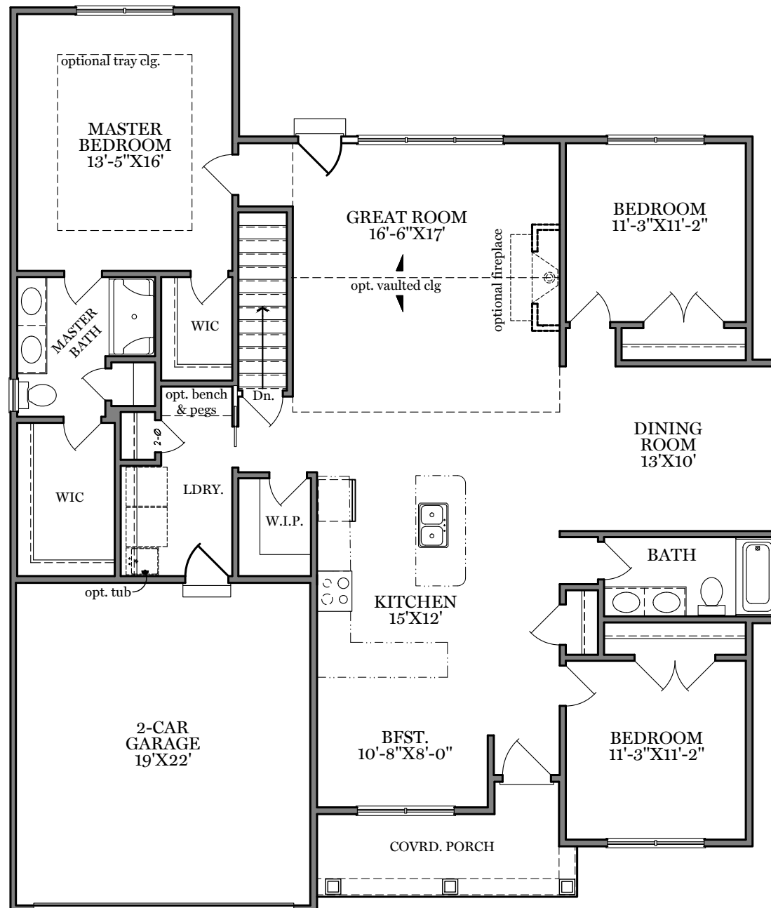
First Floor Plan - 1,829 sf "HENSLEY"
