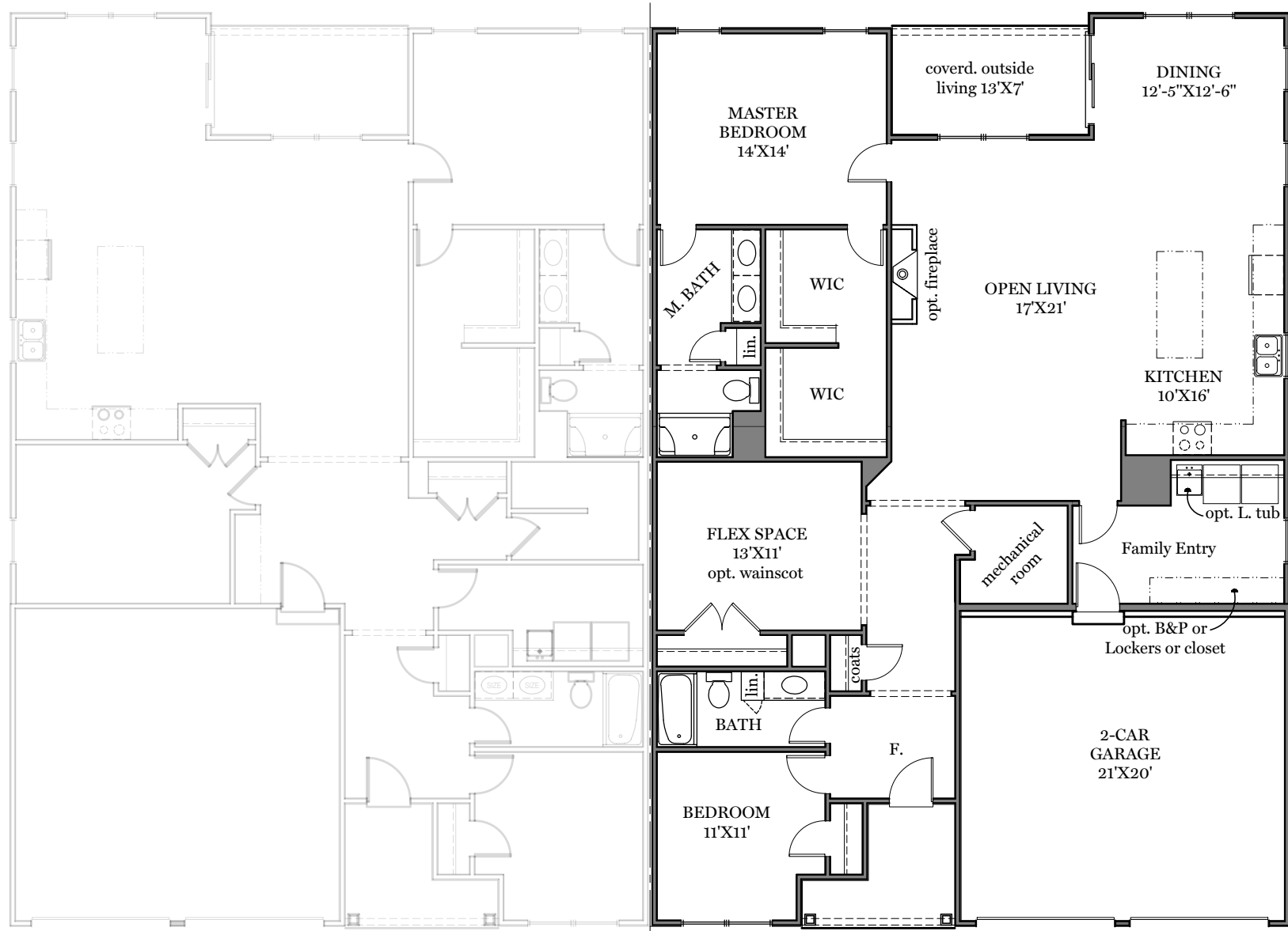
First Floor Plan - 1,892 sf "CARAWAY" (slab foundation shown)
