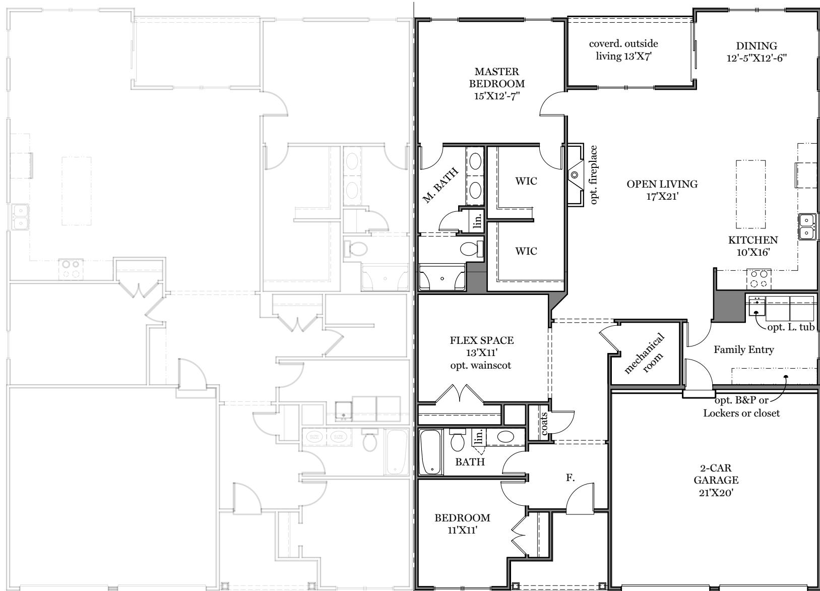
First Floor Plan - 1,892 sf "CARAWAY" (slab foundation shown)
