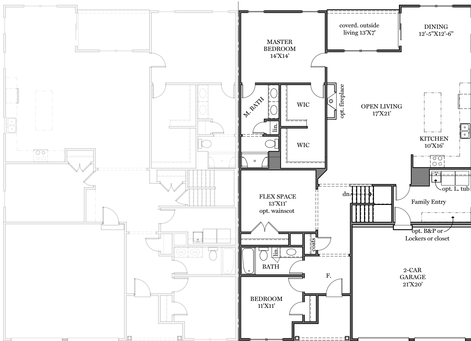
First Floor Plan - 1,892 sf "CARAWAY" (full basement option shown)
