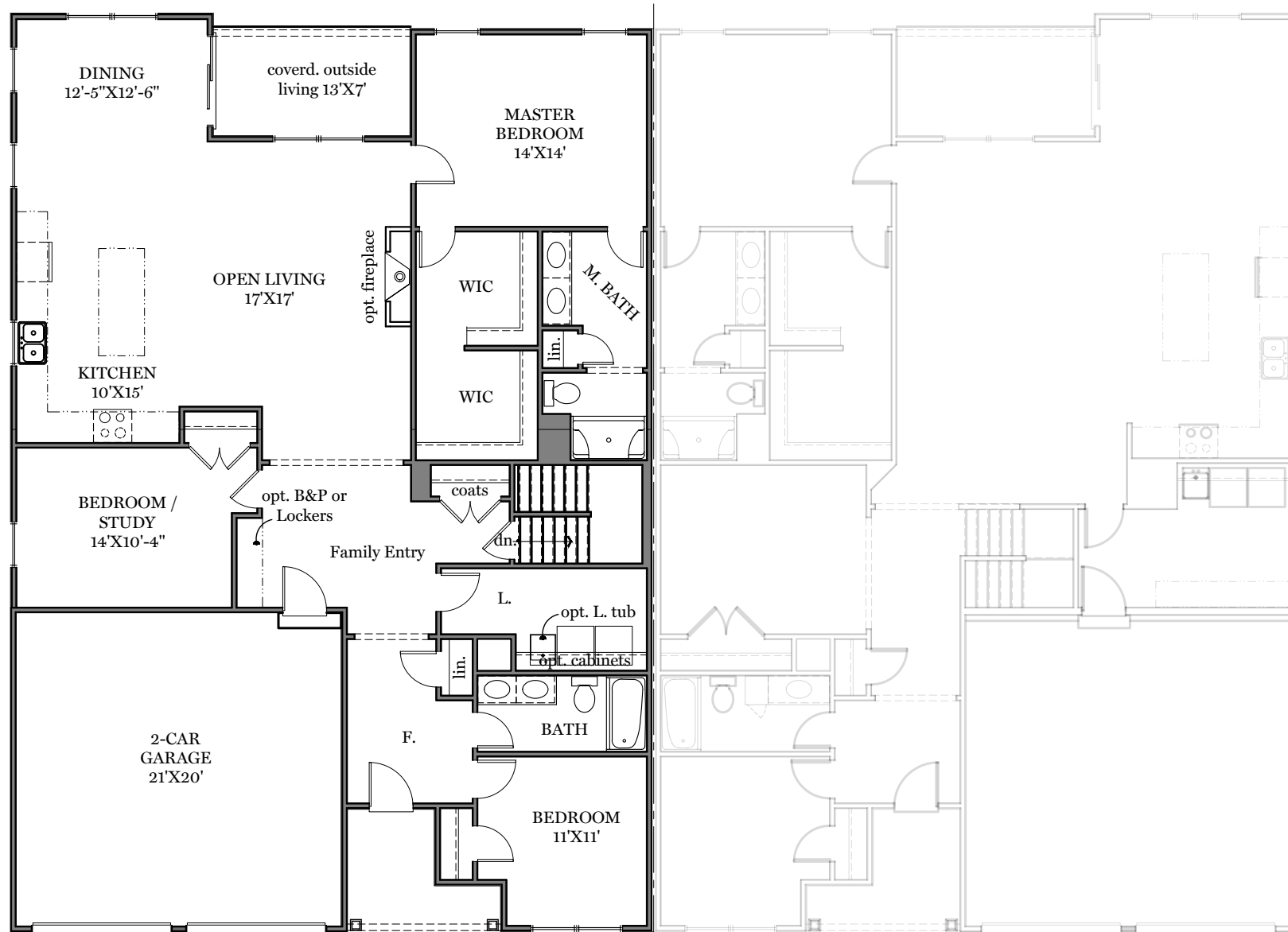
First Floor Plan - 1,892 sf "SAFFRON" (full basement option shown)
