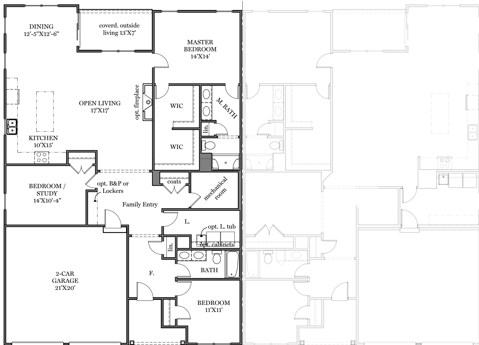
First Floor Plan - 1,892 sf "SAFFRON" (slab foundation shown)
