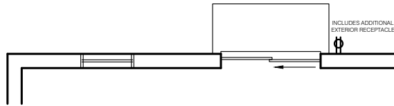
WALKOUT BASEMENT SCENARIO
