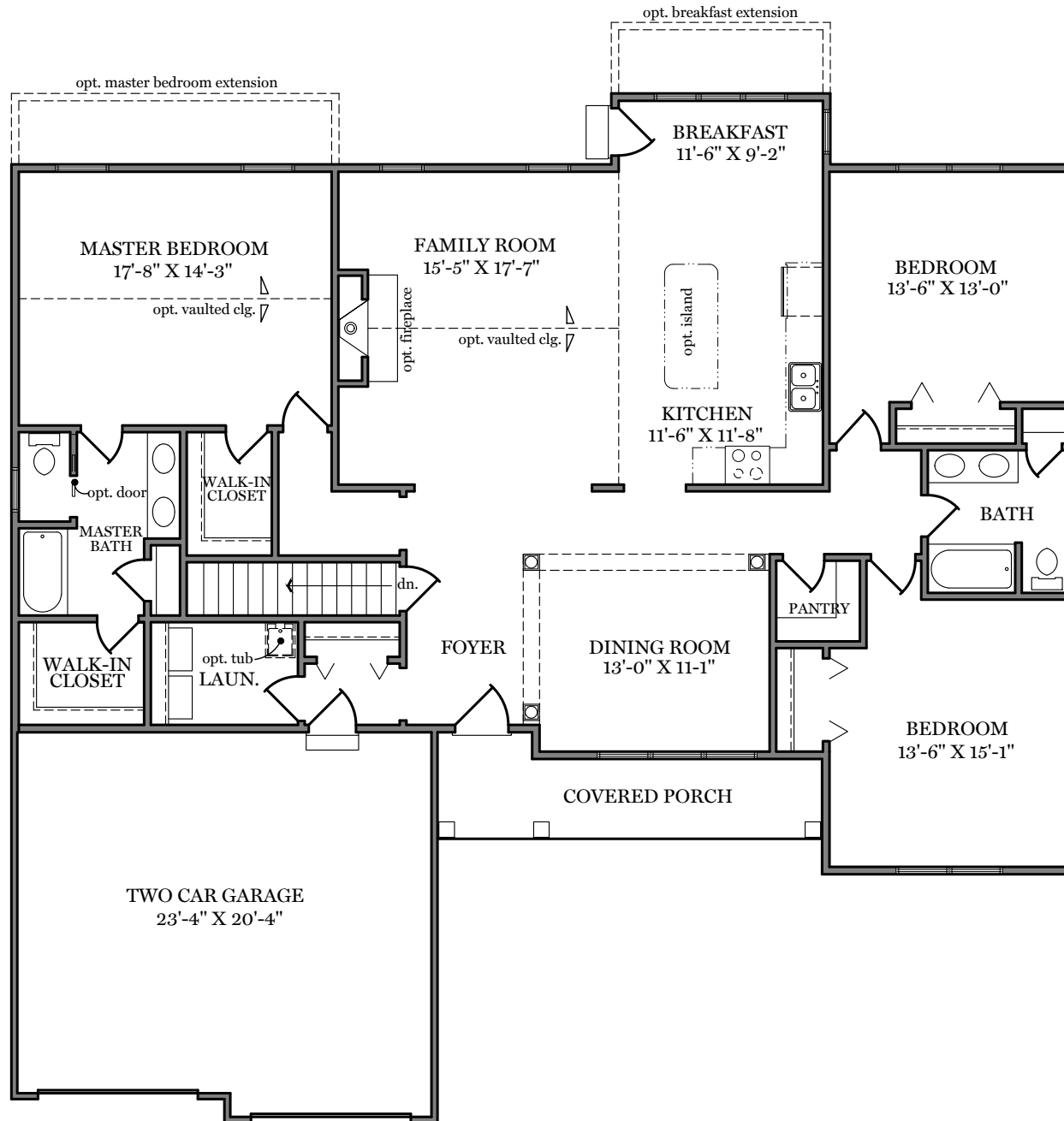
First Floor Plan - 2,108 sf "BROOKFIELD"
