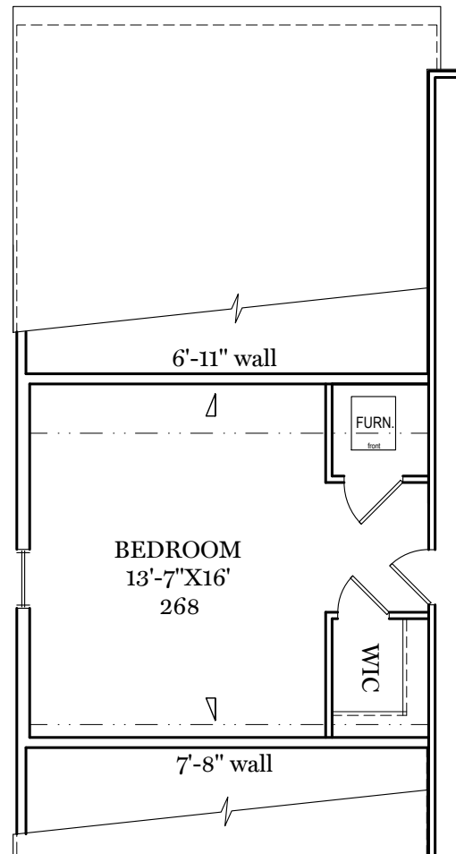
SECOND FLOOR OPTION +292 SF
