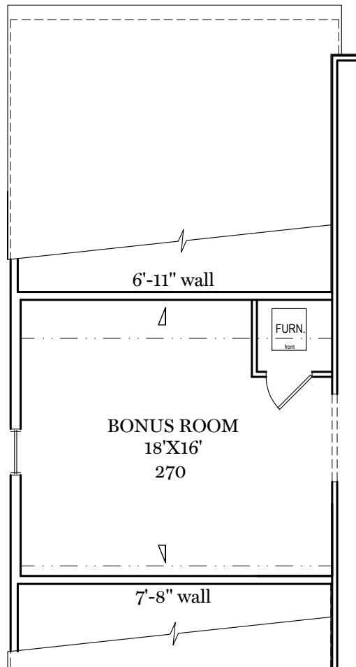
SECOND FLOOR OPTION (only with opt. office)
