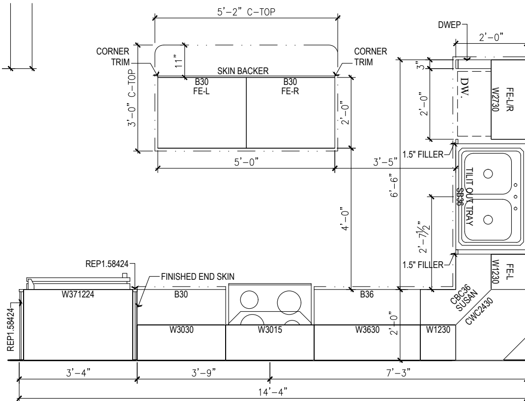
1 Kitchen Cabinet Plan
