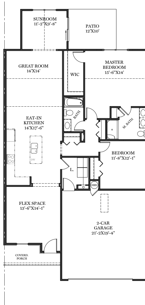
1st Floor Plan - 1,598 sf "FERRIS"
