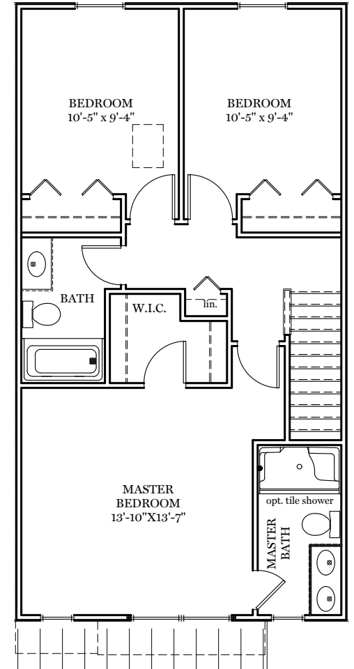
Upper Floor Plan - 737 sf
