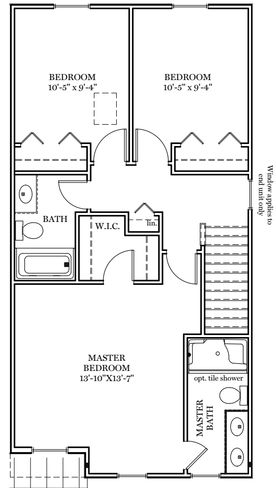
Upper Floor Plan - 768 sf
