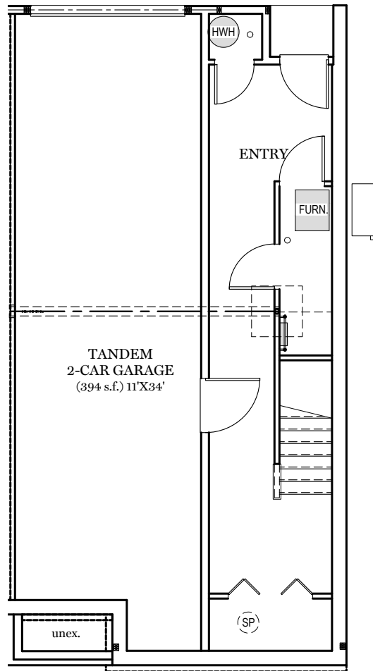
Lower Floor Plan - 320 sf
