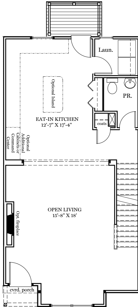
Living Floor Plan - 762 sf
