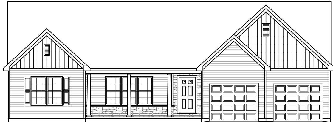
CLASSIC ELEVATION
