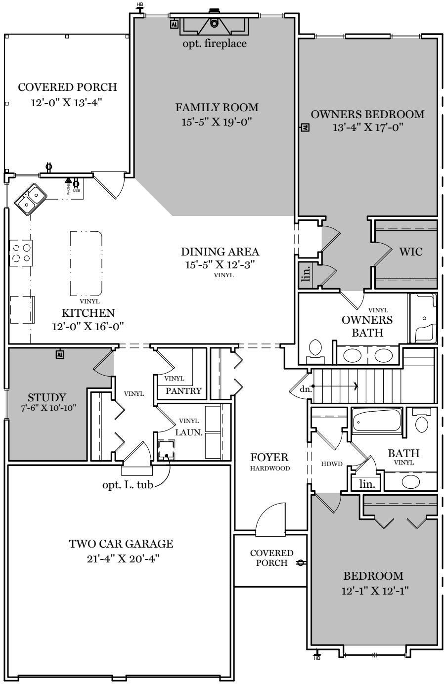
1st Floor Plan - 1,892 sf
