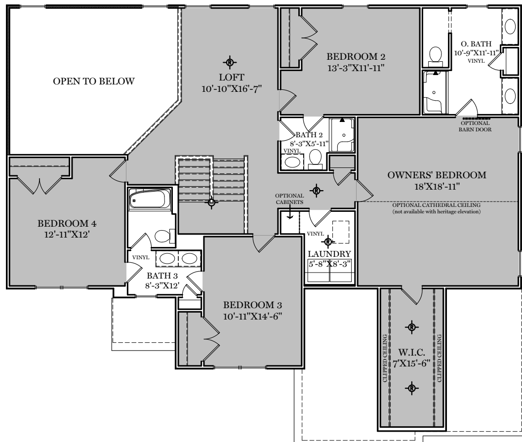
OPTIONAL 2-STORY FAMILY ROOM (REMOVES 308 SF)
