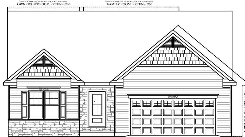
AMERICAN ELEVATION
