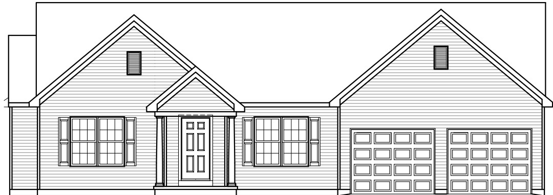
TRADITIONAL ELEVATION**
