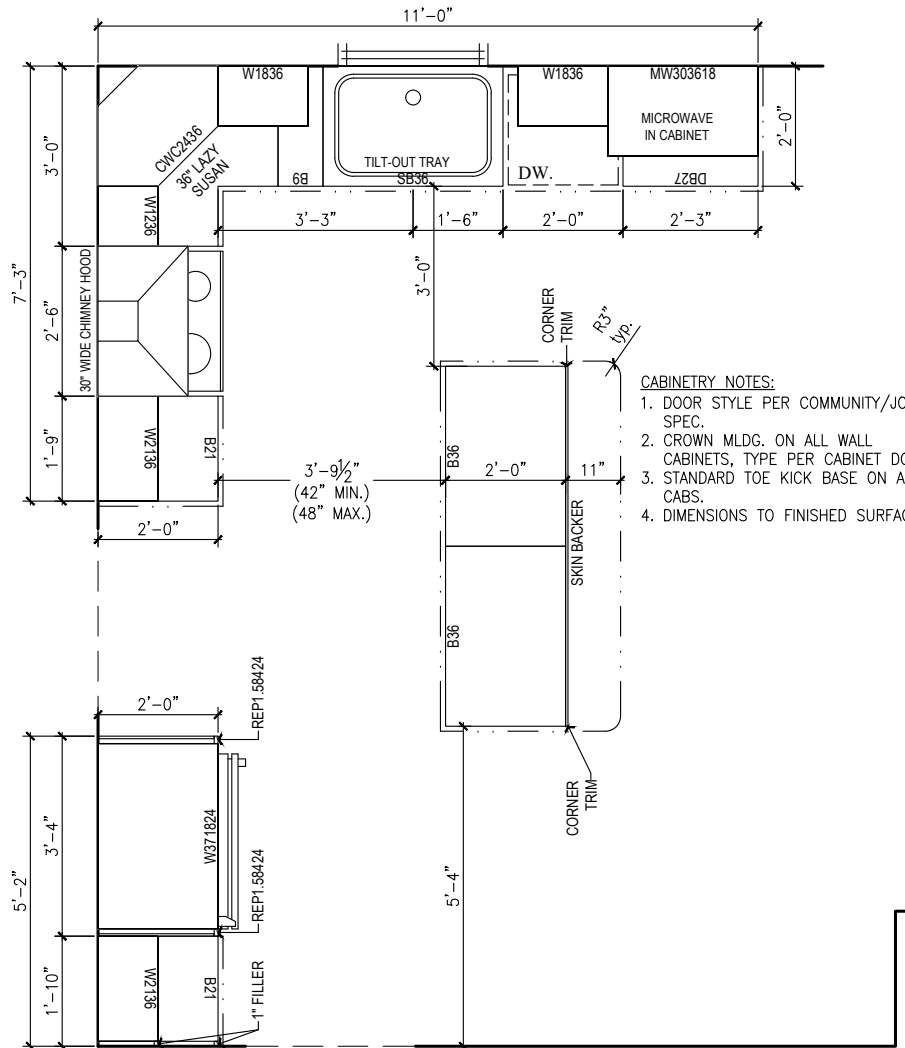
1 Kitchen Cabinet Plan
