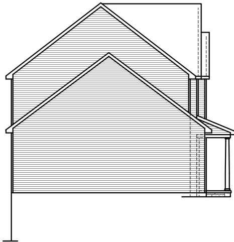
left elevation
