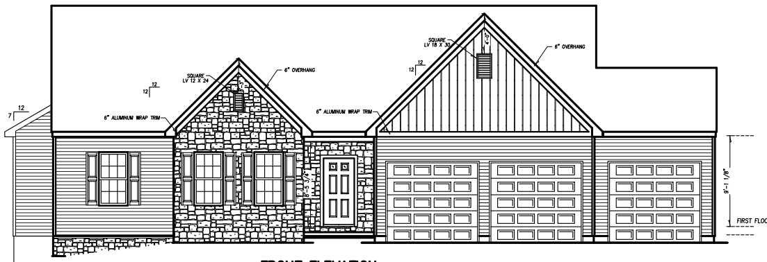
FRONT ELEVATION
