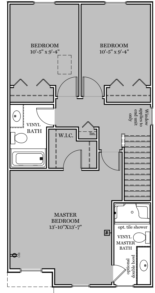
Upper Floor Plan - 768 sf
