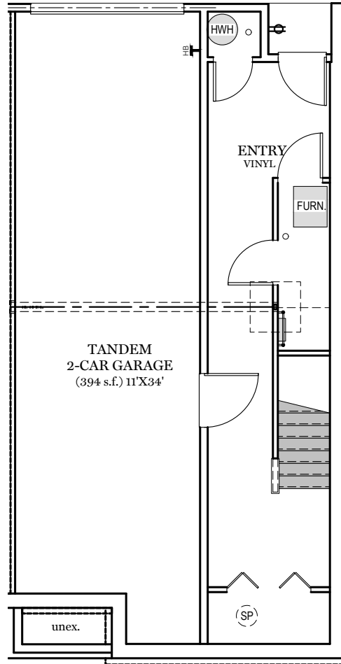
Lower Floor Plan - 320 sf
