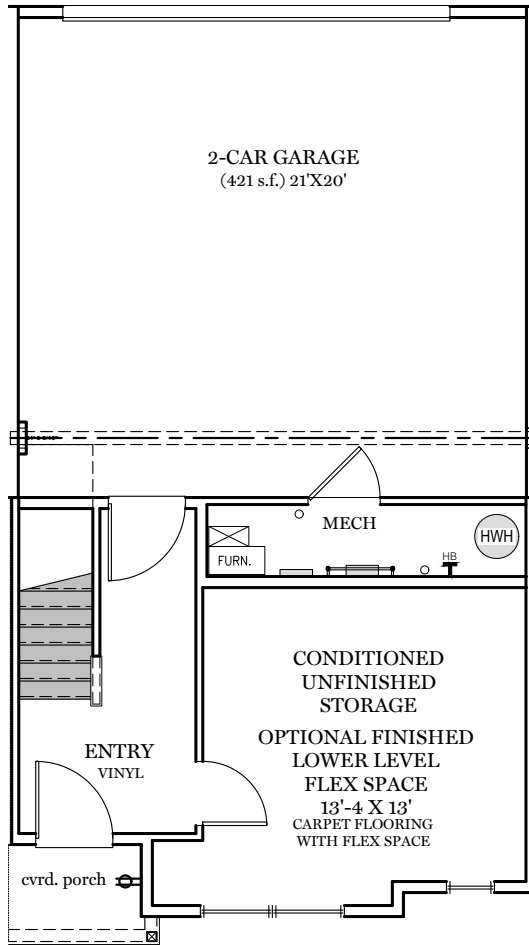
Lower Floor Plan - 87 sf
