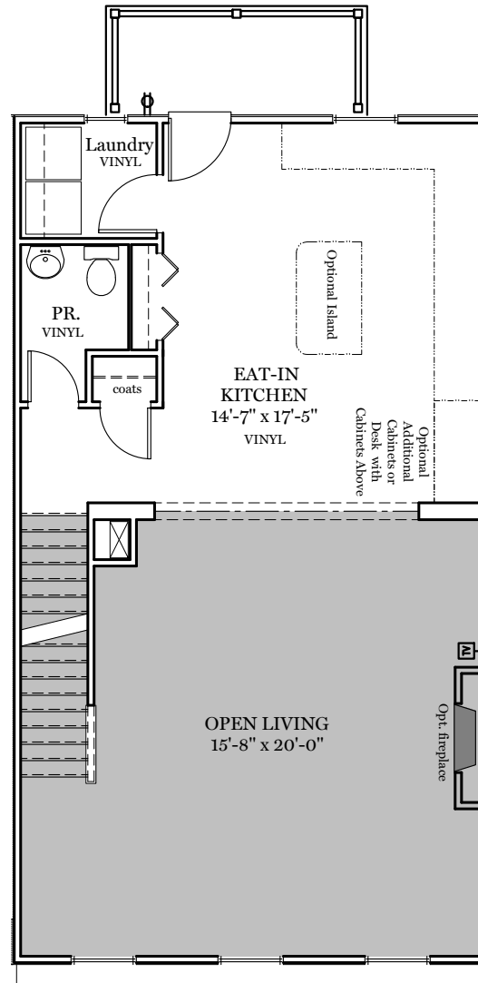
Living Floor Plan - 858 sf
