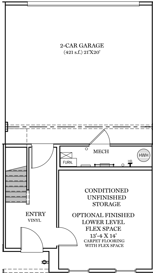
Lower Floor Plan - 94 sf
