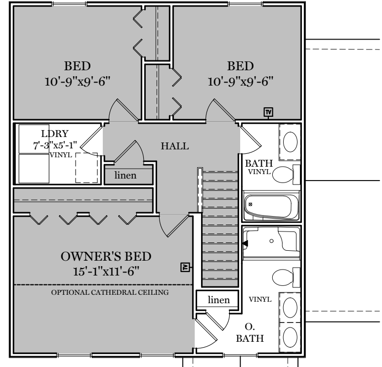
OPTIONAL SECOND FLOOR PLAN (LARGER LAUNDRY & ADDITIONAL LINEN CLOSET) TRADITIONAL** FLOOR PLAN SHOWN
