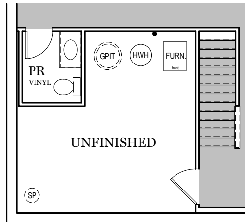
OPTIONAL FINISHED POWDER ROOM (+36 SF)
