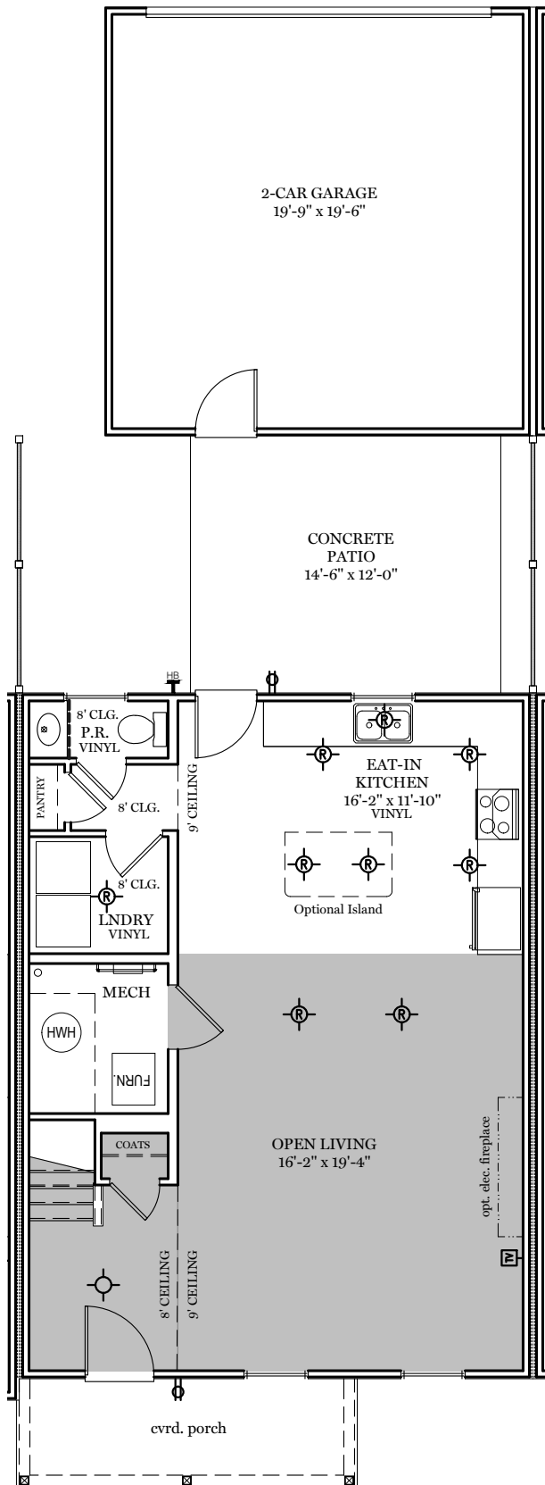
Living Floor Plan - 768 sf
