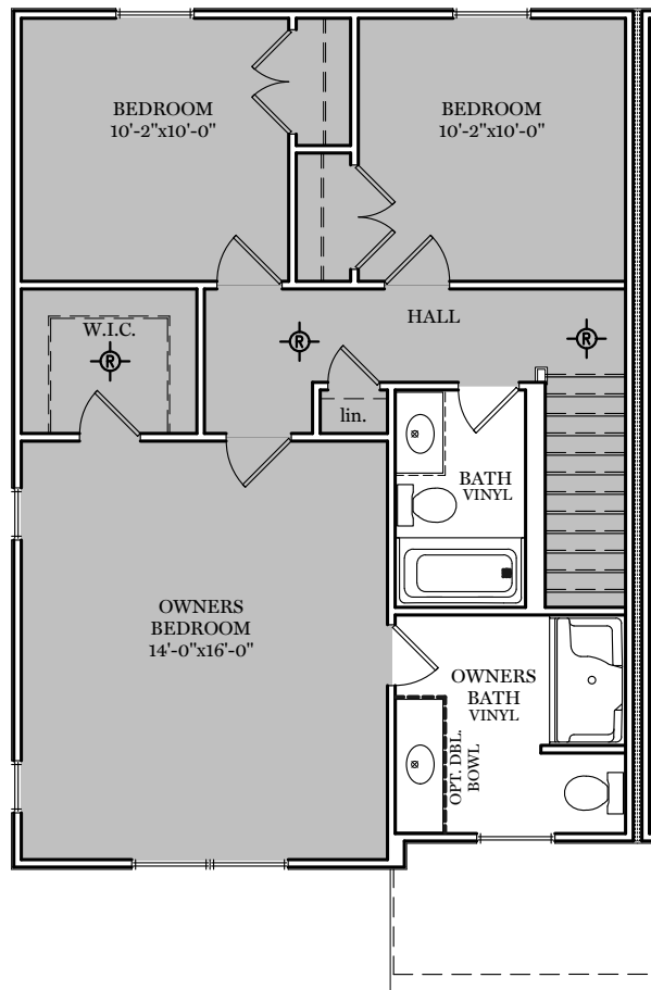
Upper Floor Plan - 783 sf
