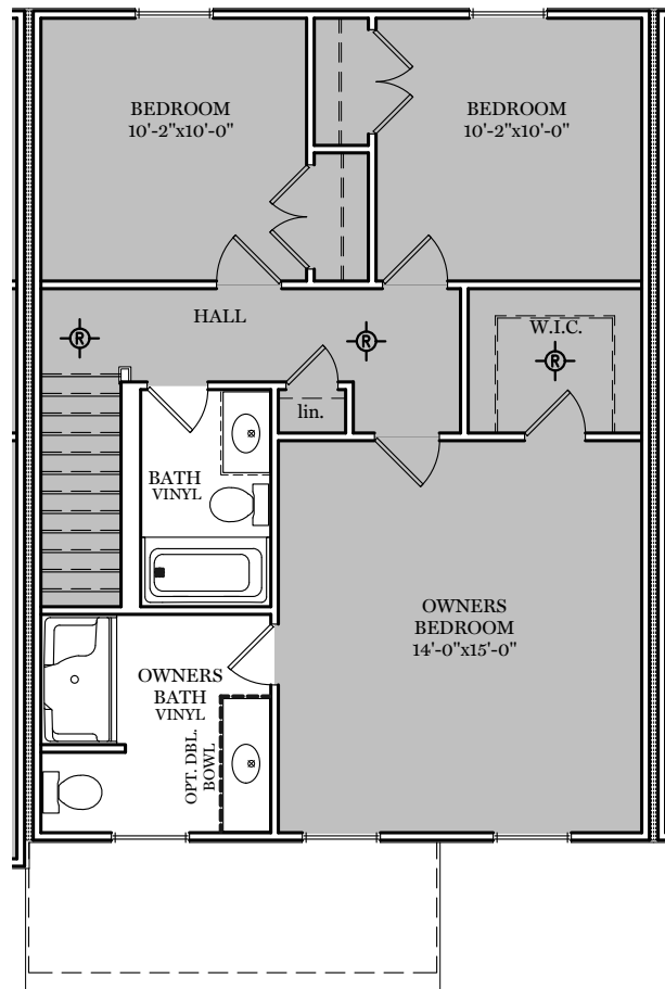
Upper Floor Plan - 768 sf
