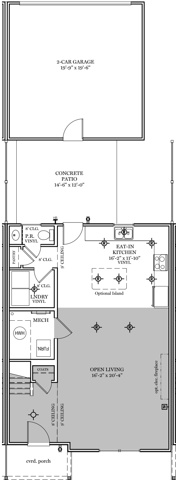
Living Floor Plan - 783 sf
