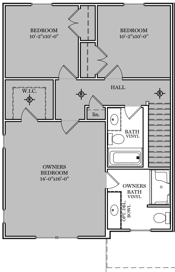
Upper Floor Plan - 783 sf
