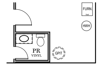
OPTIONAL FINISHED POWDER ROOM (+ 36 SF)
