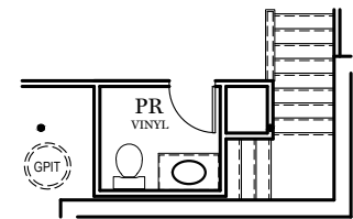
OPTIONAL FINISHED POWDER ROOM (+41 SF)
