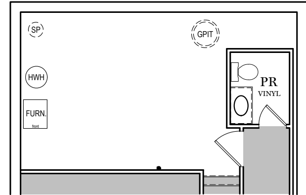
OPTIONAL FINISHED POWDER ROOM (+56 SF)
