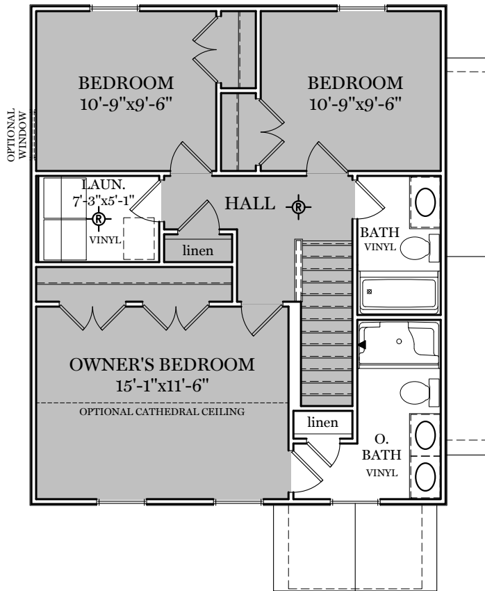
OPTIONAL SECOND FLOOR PLAN (LARGER LAUNDRY & ADDITIONAL LINEN CLOSET) TRADITIONAL** FLOOR PLAN SHOWN
