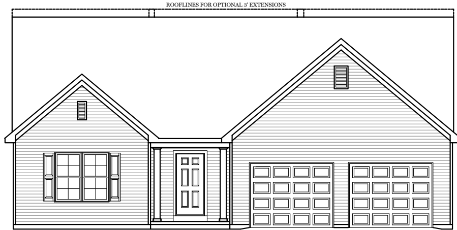
TRADITIONAL ELEVATION**
