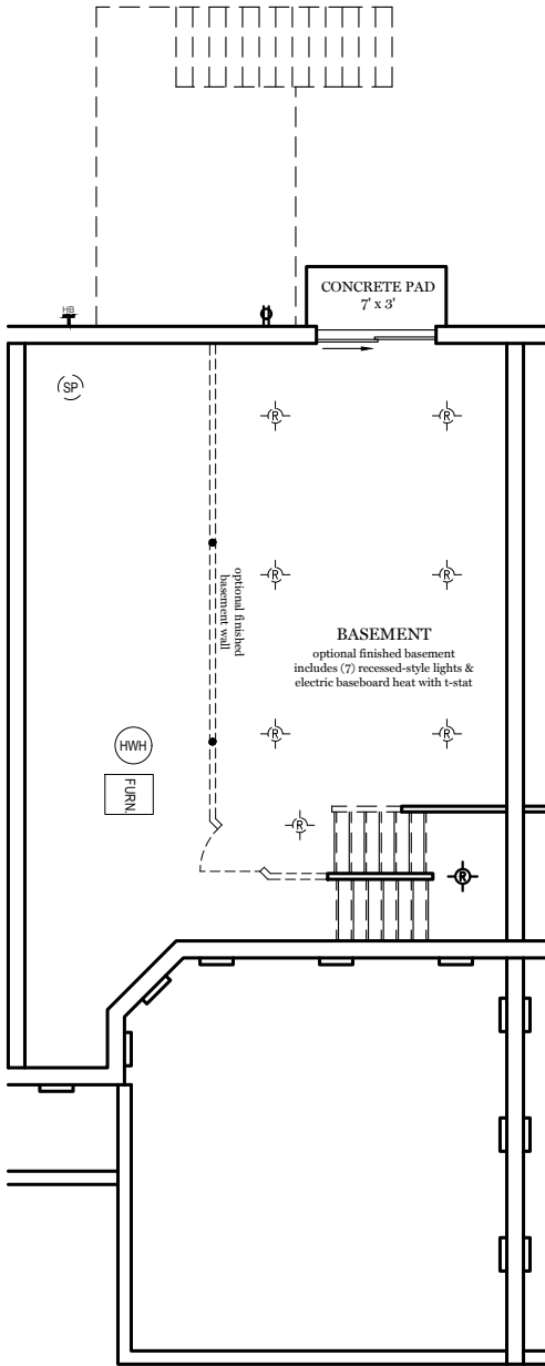
Lower Floor Plan (optional 423 SF finished space)
