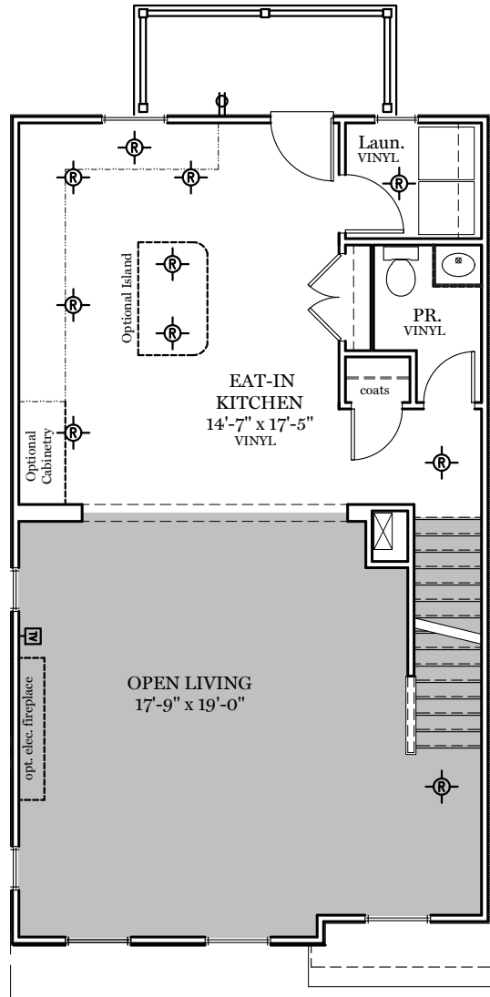
Living Floor Plan - 827 sf
