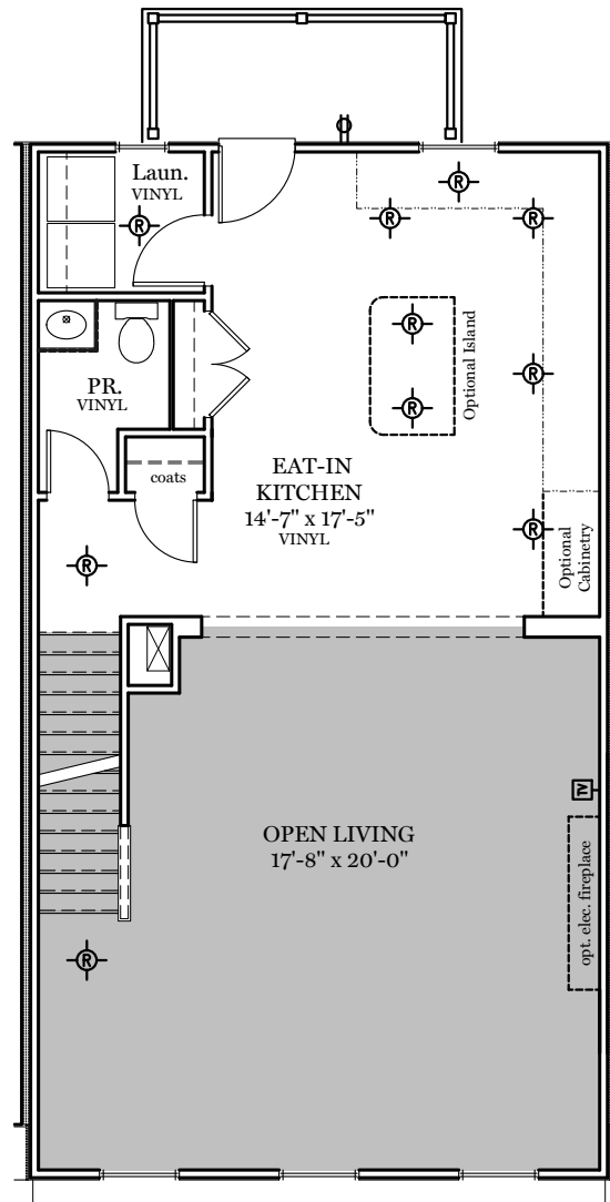
Living Floor Plan - 858 sf
