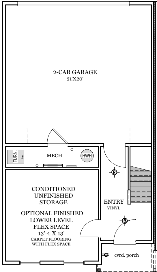
Lower Floor Plan - 87 sf
