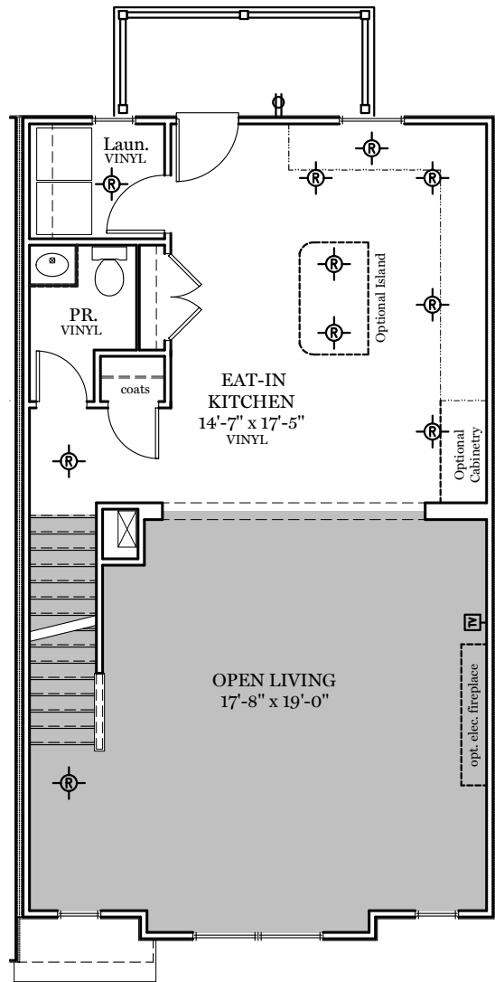
Living Floor Plan - 825 sf
