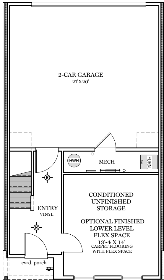
Lower Floor Plan - 94 sf
