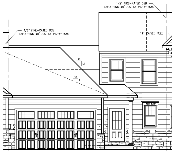
FRONT ELEVATION
