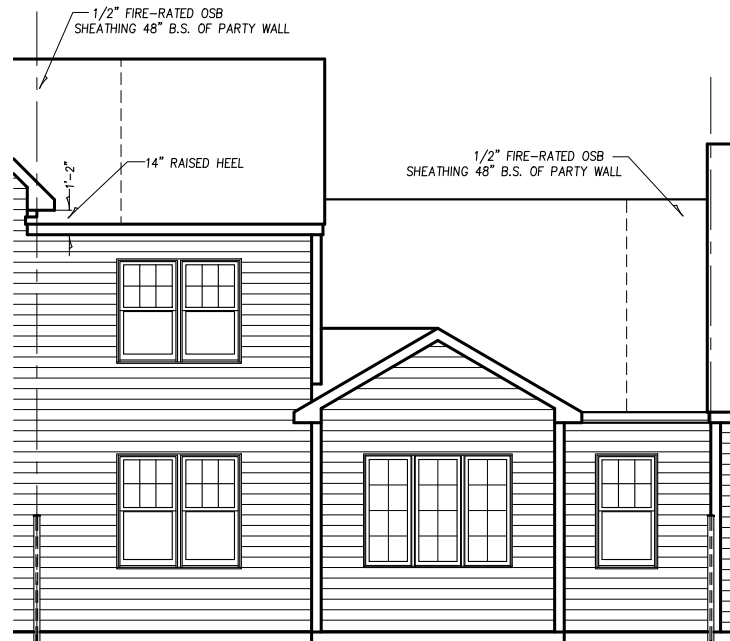
REAR ELEVATION
