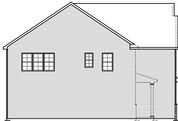
left elevation
