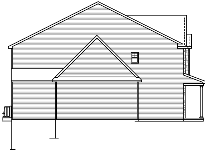
left elevation
