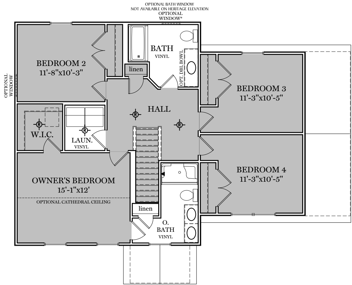
OPTIONAL 4-BEDROOM SECOND FLOOR PLAN ADDS 308 SF TRADITIONAL** FLOOR PLAN SHOWN
