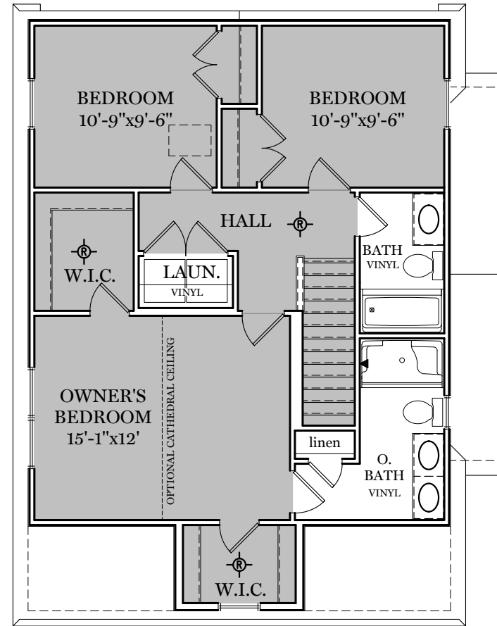
HERITAGE FLOOR PLAN
