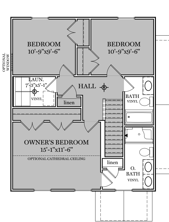
OPTIONAL SECOND FLOOR PLAN (LARGER LAUNDRY & ADDITIONAL LINEN CLOSET) TRADITIONAL** FLOOR PLAN SHOWN
