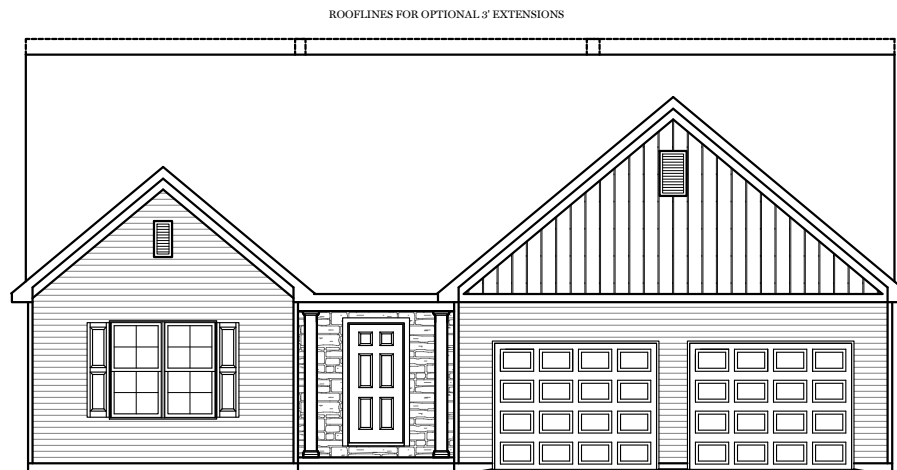
CLASSIC ELEVATION
