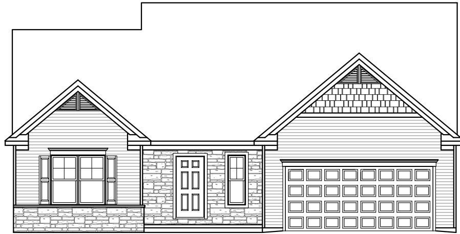
AMERICAN ELEVATION
