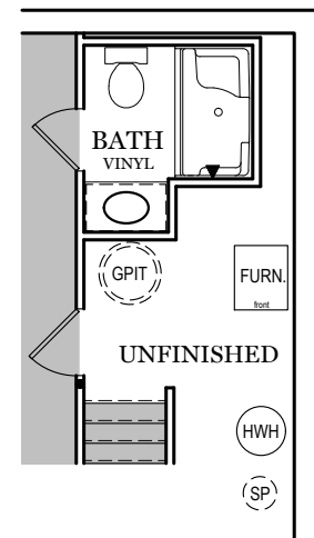
OPTIONAL FINISHED BATHROOM (+44 SF)
