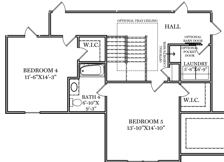
OPTIONAL 5TH BEDROOM AND 4TH BATH (LEGACY FLOOR PLAN SHOWN) **NOT AVAILABLE WITH 2-STORY FAMILY ROOM**
