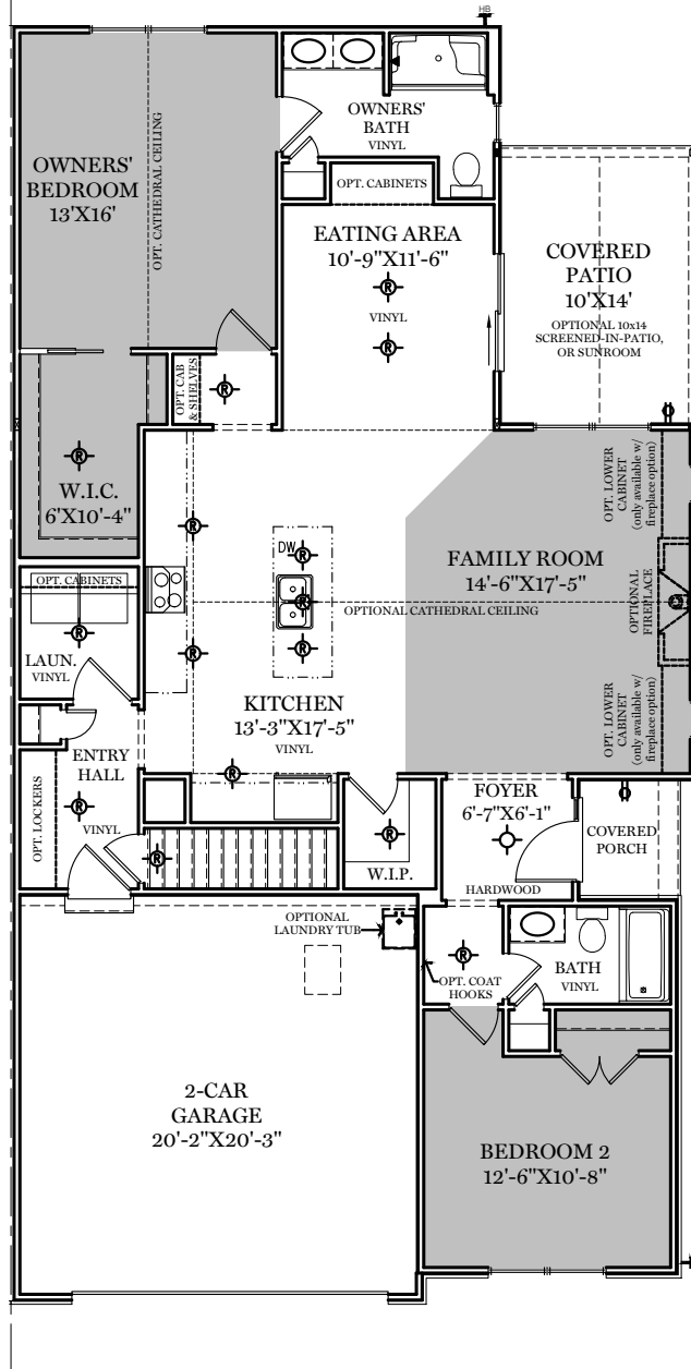
1st Floor Plan - 1,572 sf HAWTHORNE I
