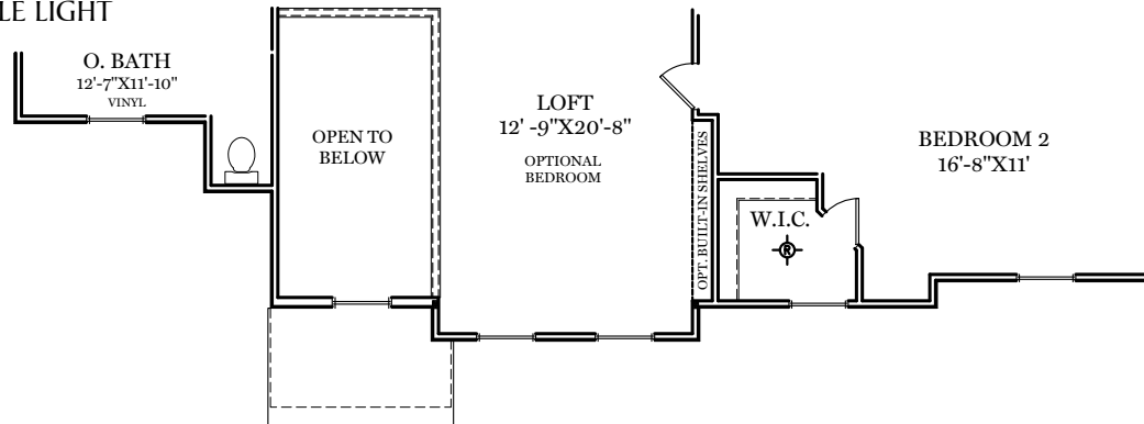
CLASSIC FLOOR PLAN
